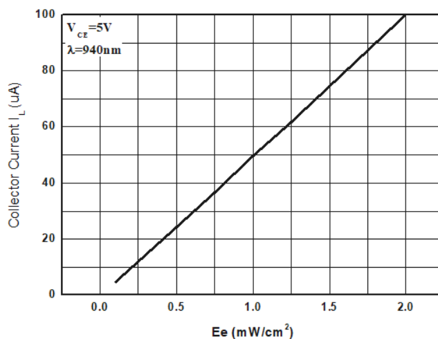
Fig. 2 Reverse Light Current vs. Ee
