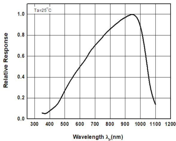
Fig.1 Spectral Sensitivity
