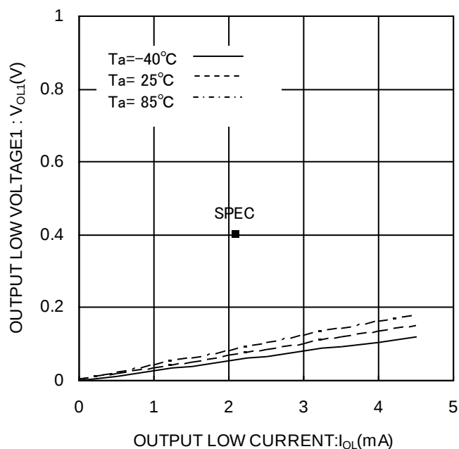
Figure 6. Output low voltage1 V_{OL1} (VCC=2.7V)
