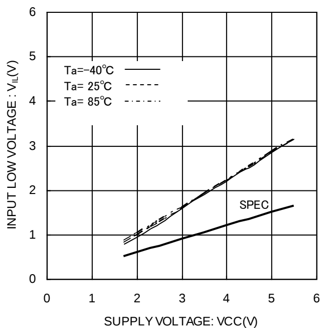
Figure 5. Input low voltage V_{IL} (CS,SK,DI)
