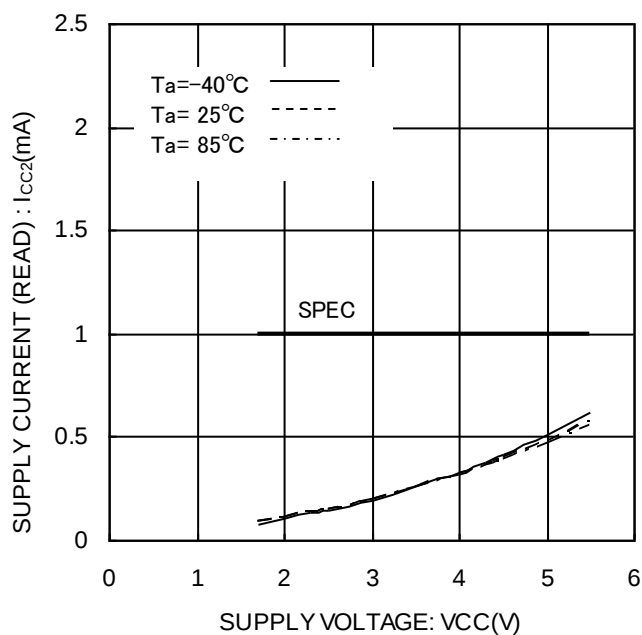
Figure 17. Supply current (READ) I_{CC2}(\text{READ}, f_{SK}=3\text{MHz})
