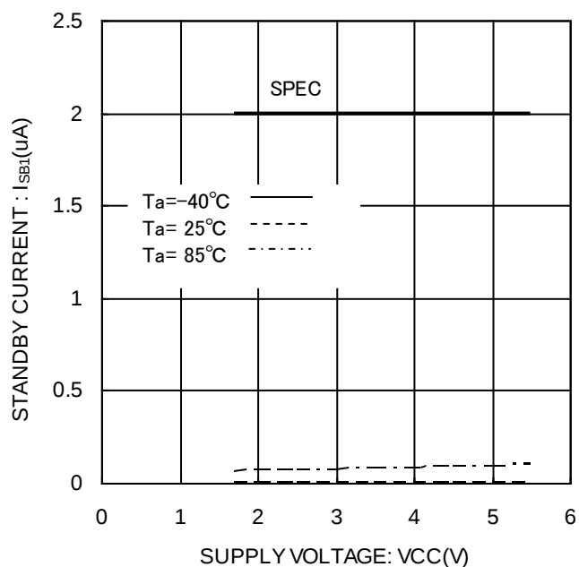
Figure 20. Standby current I_{SB1}(CS=0V)
