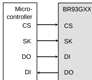
(a). Connection by 4 lines
