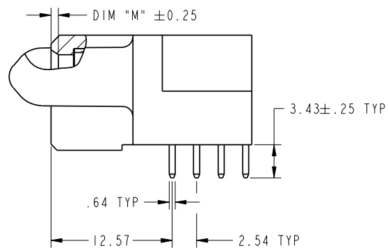
SECTION F-F SCALE 2:1
