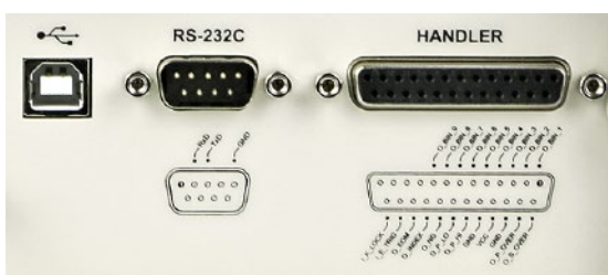
Standard Interface
