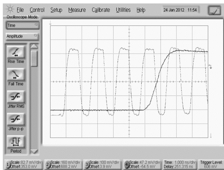
SY88149NDL Input Preamble burst with Signal Detect (SD) Response, with Noise Discriminator engaged
