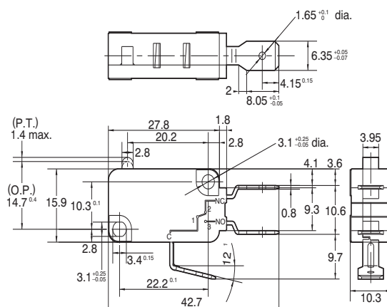
.250 Quick-connect terminal
