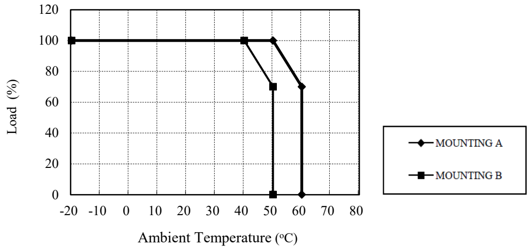
Derating Curve
