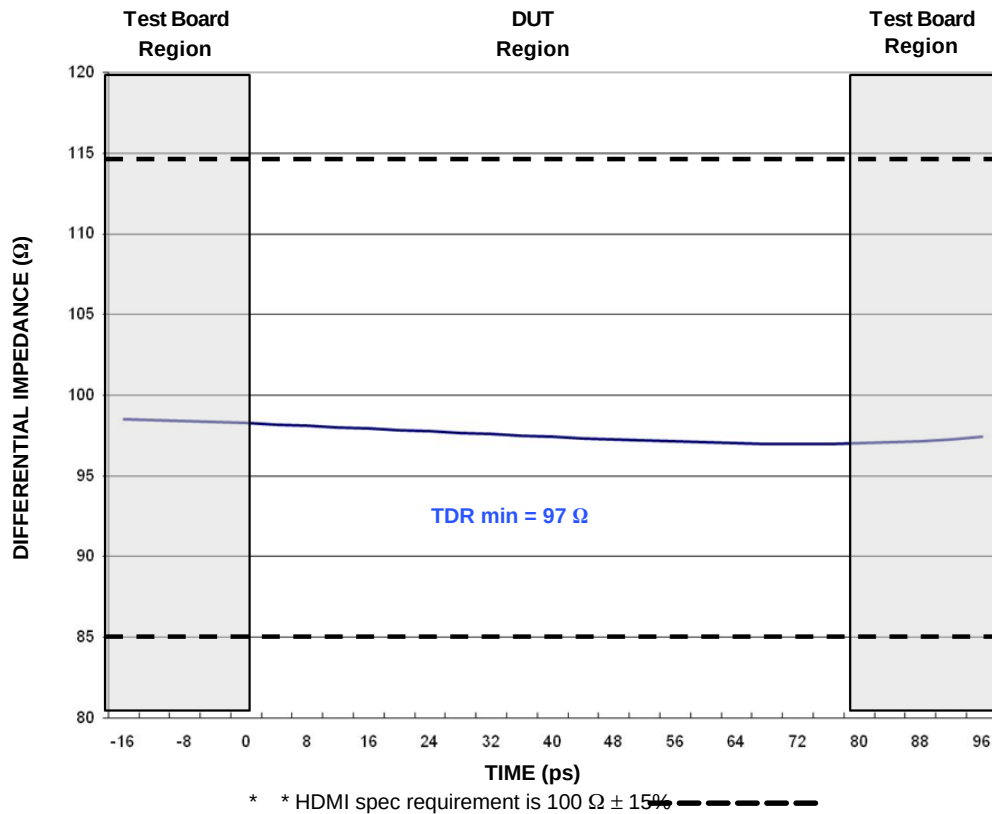
Figure 22. HDMI TDR Measurement. 100 \Omega Differential Impedance Target, 200 ps Rise Time
