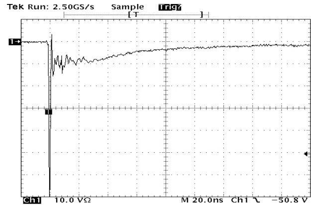
Figure 8. IEC61000-4-2 -8 KV Contact Clamping Voltage
