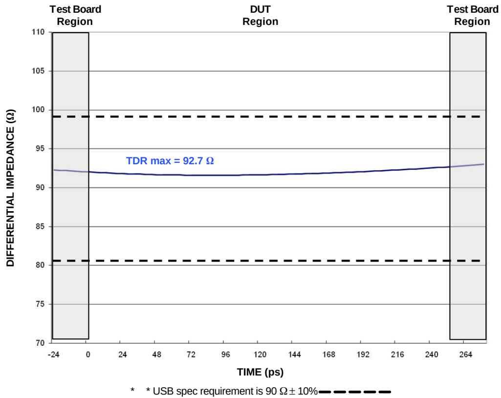
Figure 21. USB TDR Measurement. 90 \Omega Differential Impedance Target, 200 ps Rise Time
