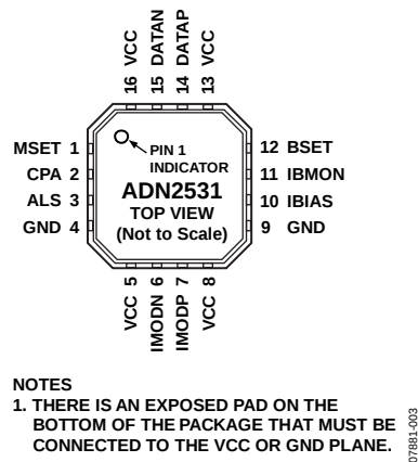
Figure 3. Pin Configuration
