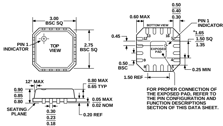
Figure 42. 16-Lead Lead Frame Chip Scale Package [LFCSP_WQ] 3 mm x 3 mm Body, Very Very Thin Quad (CP-16-27) Dimensions shown in millimeters
