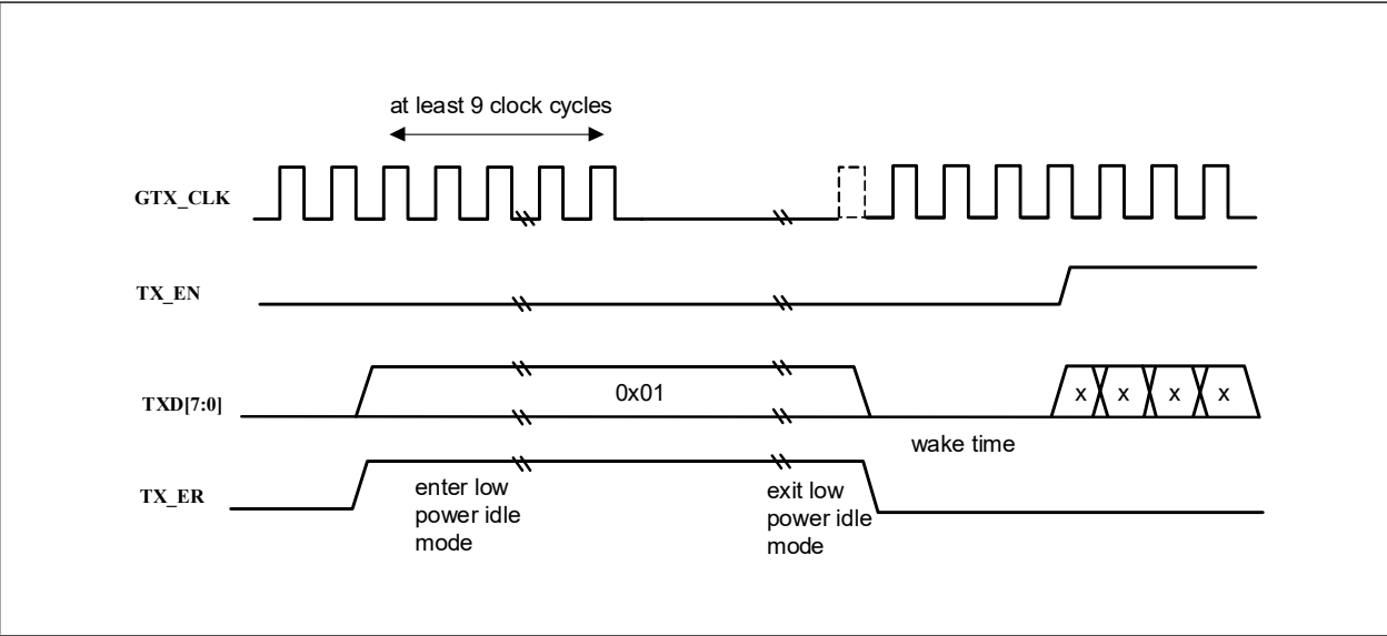
FIGURE 5-5: LPI TRANSITION - GMII (1000 MBPS) TRANSMIT
