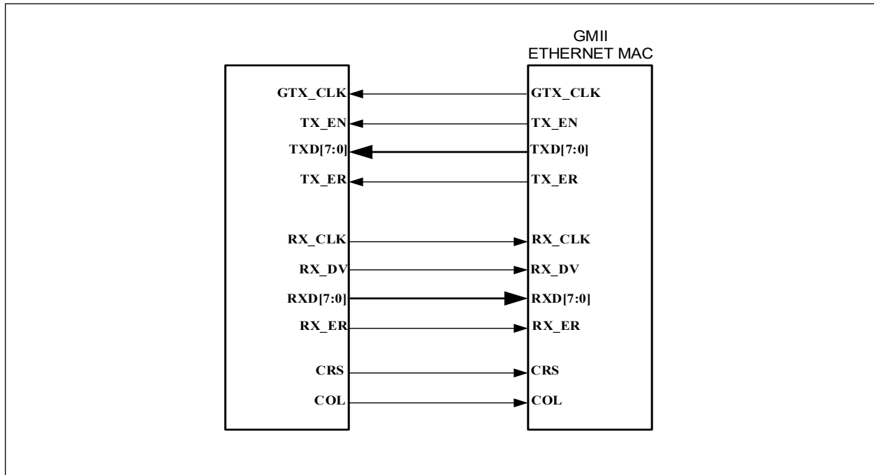
FIGURE 5-16: GMII INTERFACE
