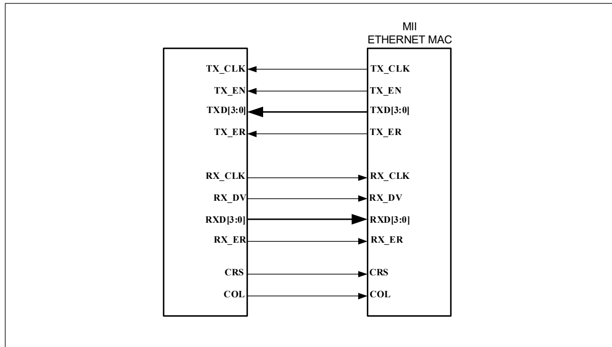
FIGURE 5-17: MII INTERFACE
