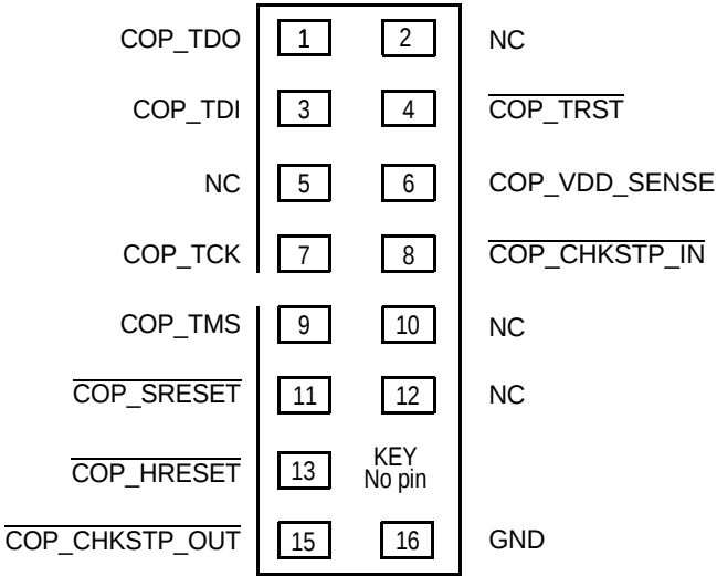
Figure 54. COP Connector Physical Pinout
