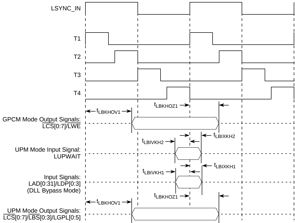
Figure 23. Local Bus Signals, GPCM/UPM Signals for LCCR[CLKDIV] = 4 or 8 (DLL Enabled)
