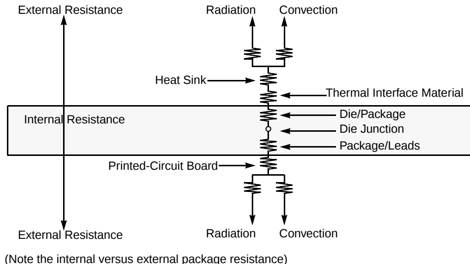
Figure 47. Package with Heat Sink Mounted to a Printed-Circuit Board
