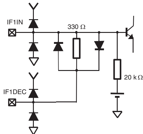
Figure 4-10. Schematic Input of the IF1 Amplifier
