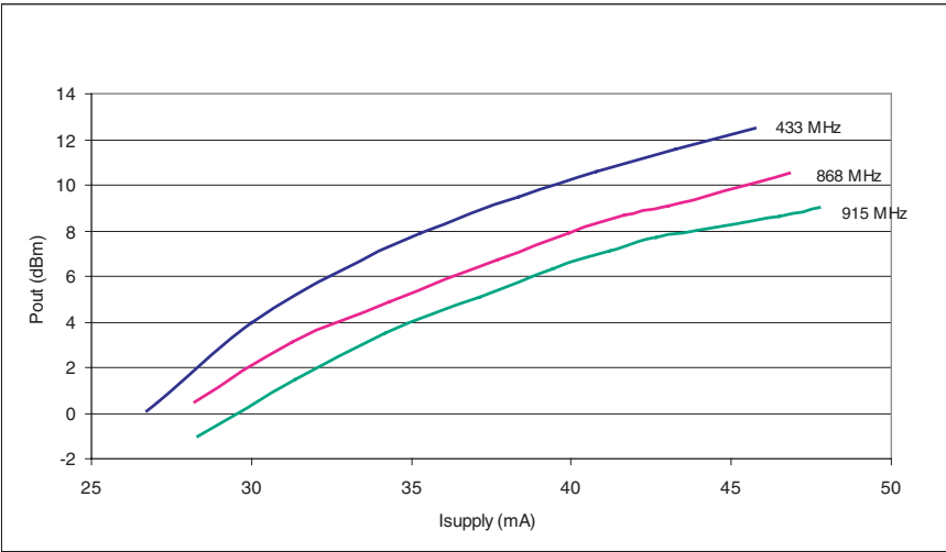
Figure 4-24. Typical Output Power of the PA for T = 25^{\circ}\text{C} and V_{CC} = 3\text{V}
