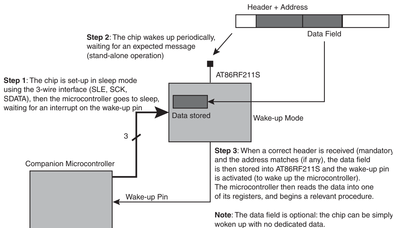
Figure 3-4. Wake-up Overview
