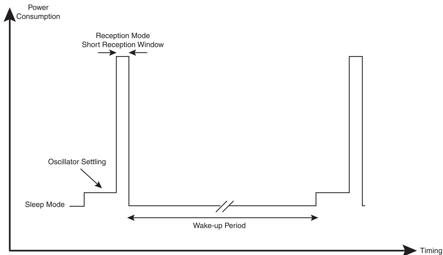
Figure 3-5. Periodical Scan
