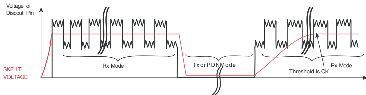
Figure 4-17. Example of Rx Timing with Discharge
