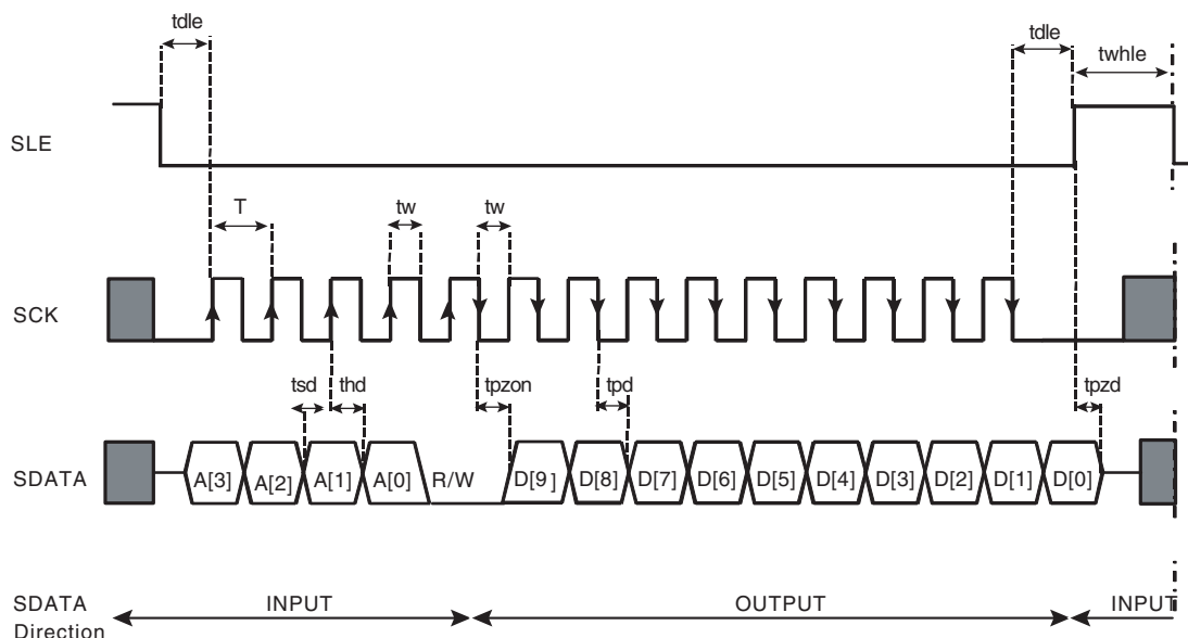
Figure 4-33. Chronogram with Timing
