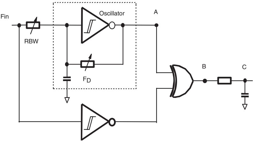
Figure 4-16. FSK Demodulator Schematic
