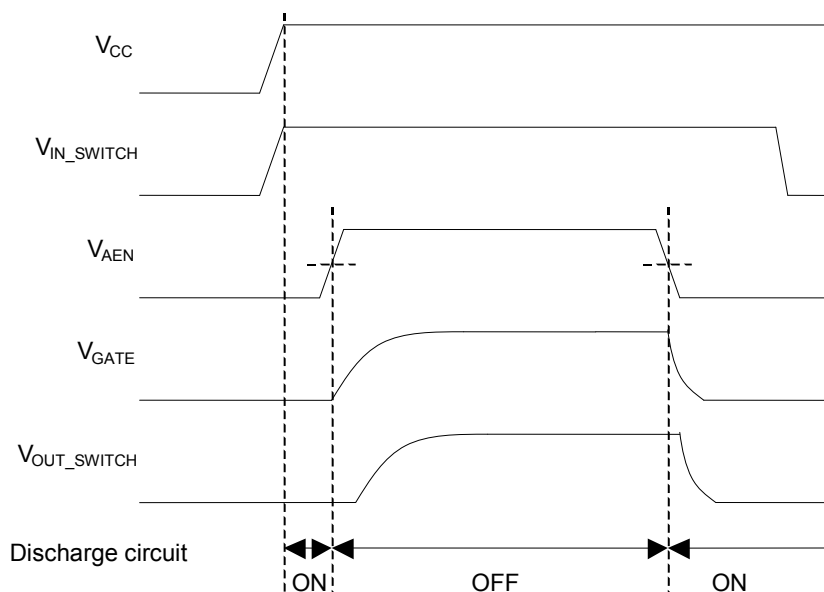
Figure 34. Operation Timing
