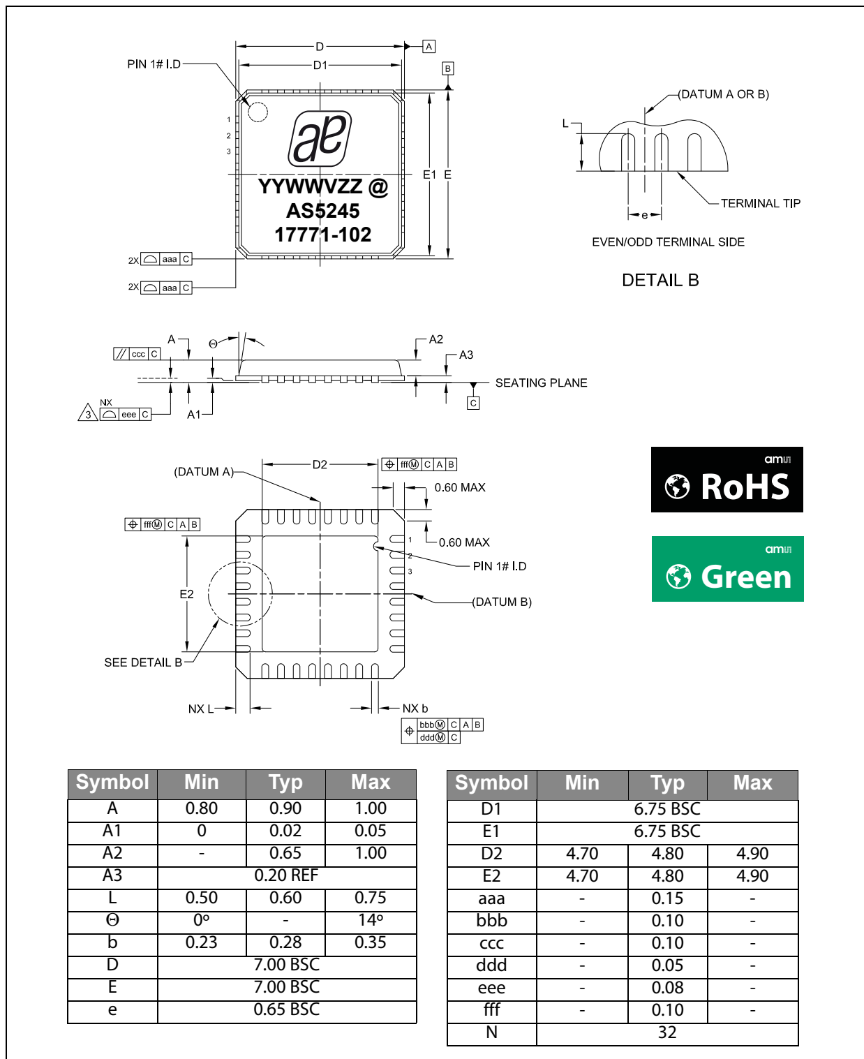
Figure 34: Package Drawing
