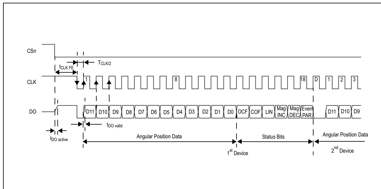
Figure 20: Daisy Chain Mode Data Transfer
