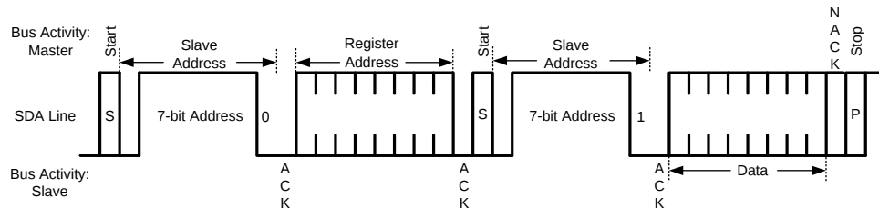
Figure 25. Read Byte
