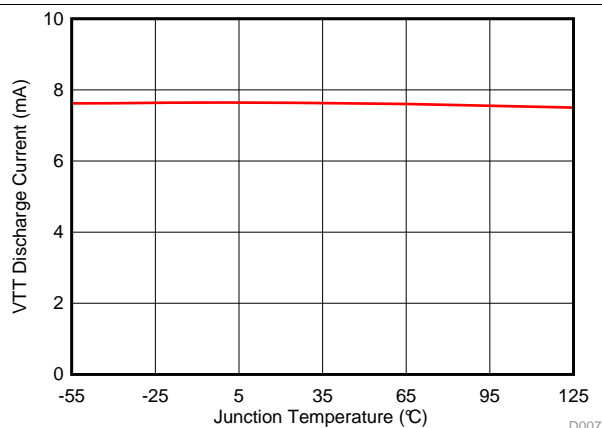
Figure 8. VTT Discharge Current vs Junction Temperature
