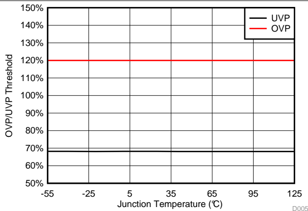
Figure 6. OVP/UVP Threshold vs Junction Temperature
