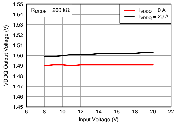
Figure 14. Line Regulation
