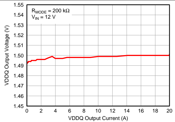
Figure 13. Load Regulation
