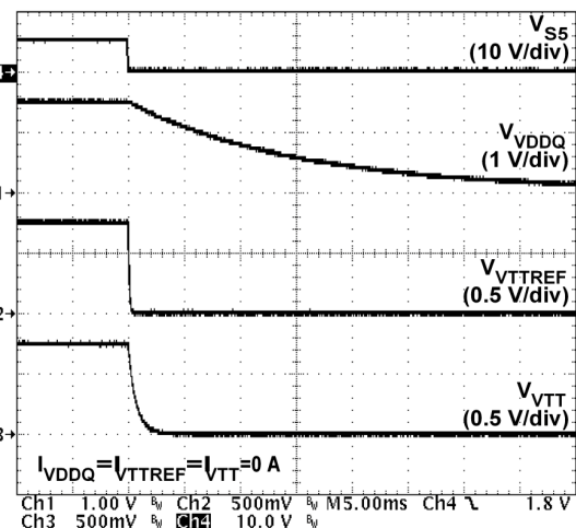
Figure 27. 1.5-V Soft-Stop Waveforms (Non-Tracking Discharge)
