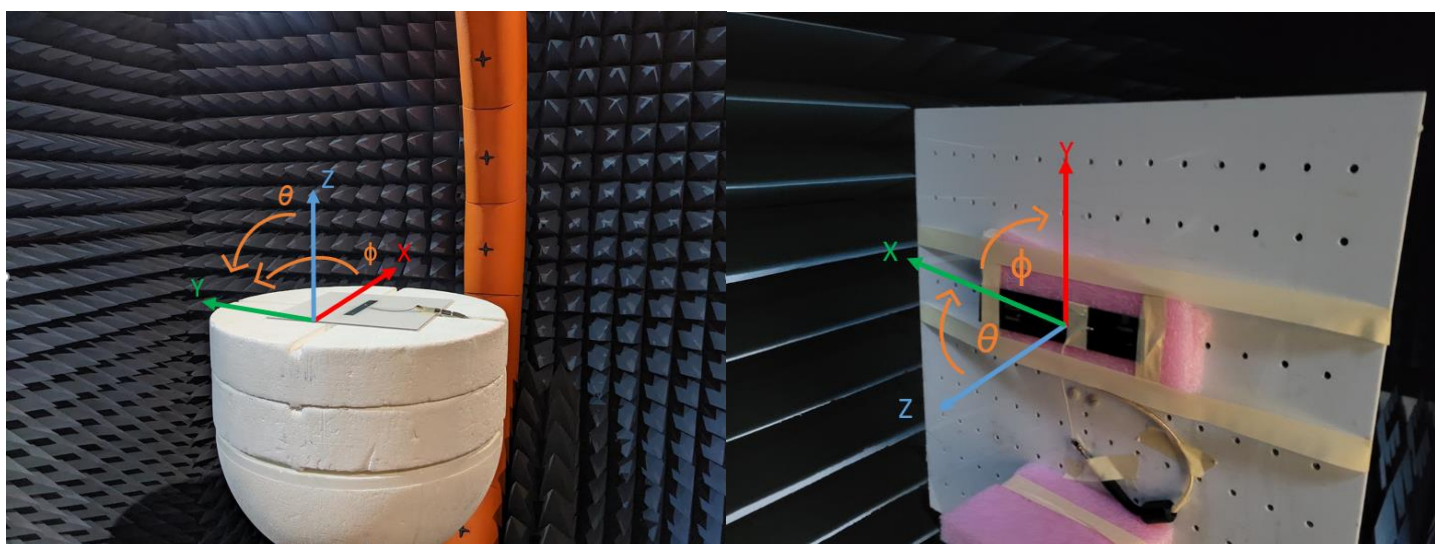
OTA Setup of the FXUB85.54.0150C in the SG24-L Satimo Test System For 600 MHz – 6 GHz Testing
