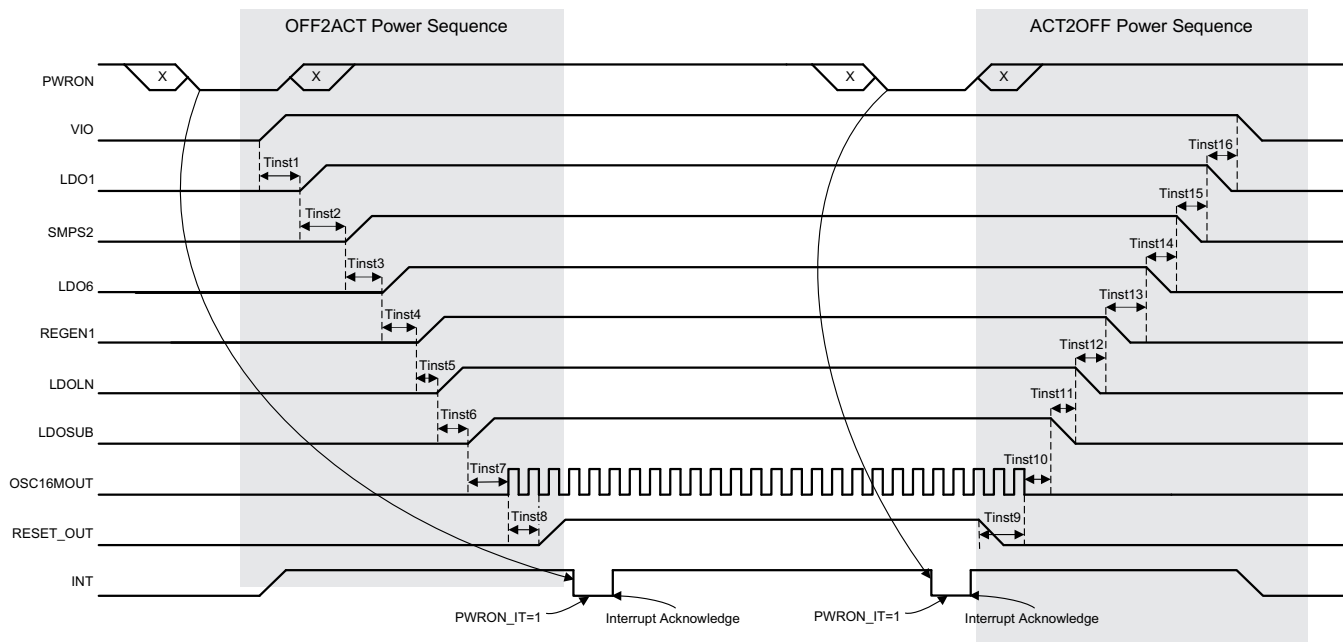
Figure 6-19. Power Sequence Example
