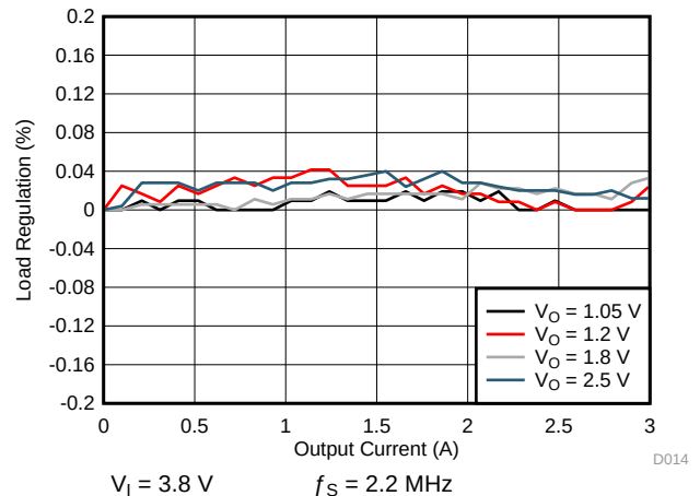
Figure 7-10. SMPS Load Regulation for 3-A Single Phase
