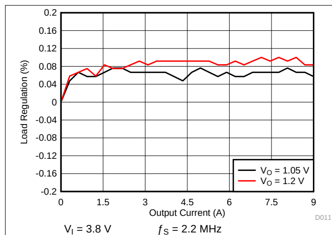
Figure 7-7. SMPS Load Regulation for 9-A Triple Phase
