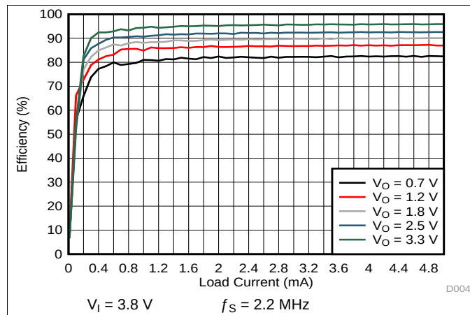
Figure 5-10. SMPS Efficiency for 2-A Single-Phase ECO-ode
