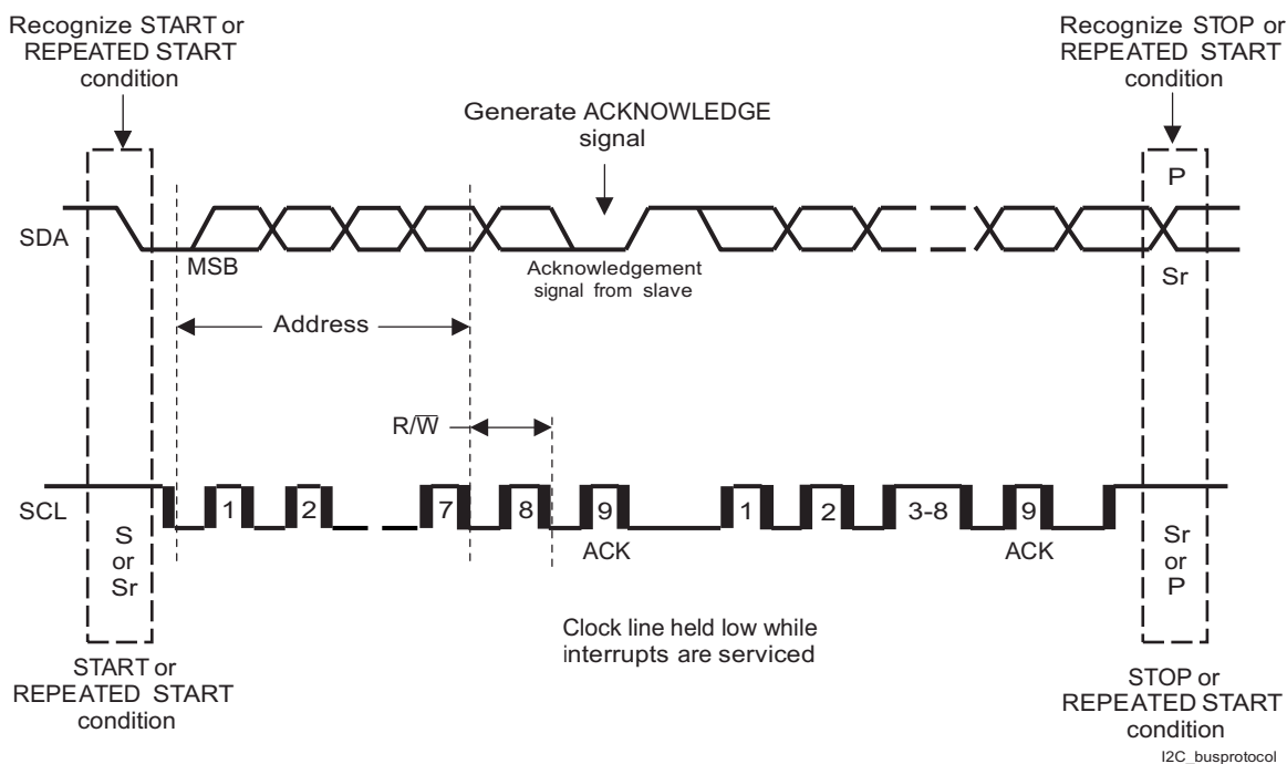
Figure 6-14. Bus Protocol
