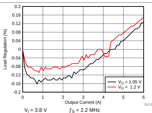
Figure 7-8. SMPS Load Regulation for 6-A Dual Phase
