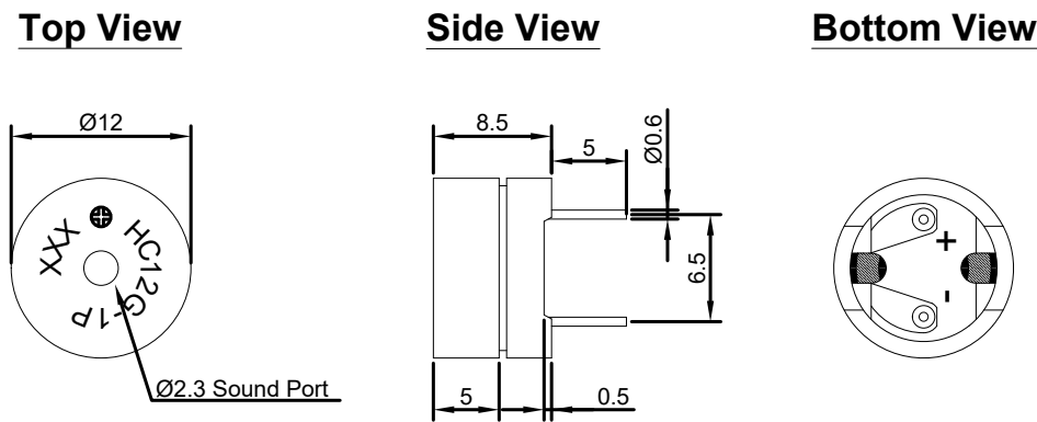
Figure 3. HC12G-1P/002 Mechanical Layout
