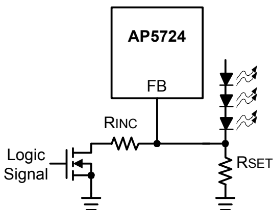
Figure 4 Dimming Control Using a Logic Signal
