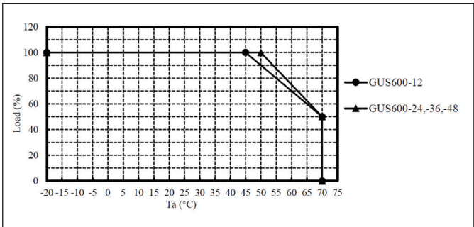
GUS600 Derating Curves vs Temperature
