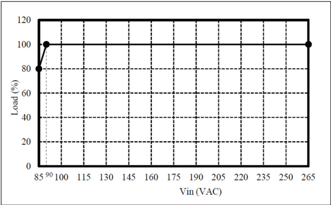
GUS600 derating Curves vs Input Voltage
