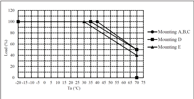
GUS350-24,-36,-48 Derating Curves vs Temperature
