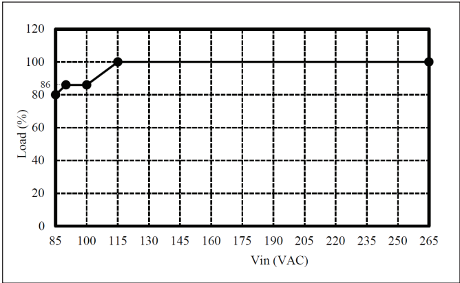
GUS1000 derating Curves vs Input Voltage
