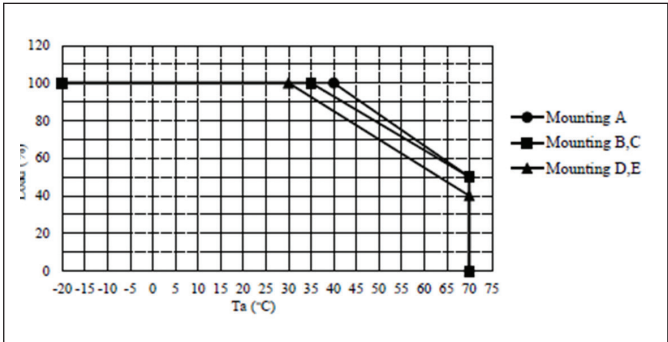
GUS600 Derating Curves vs Temperature
