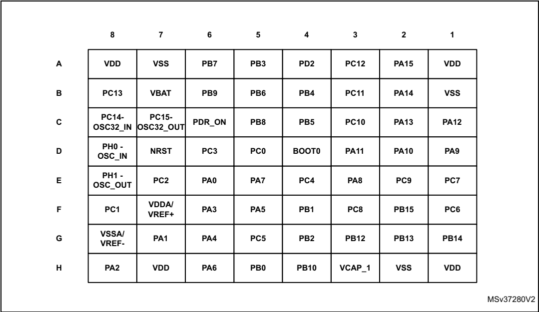
Figure 11. STM32F412xE/G WLCSP64 pinout
