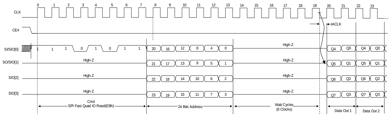
Figure 5.3 SPI Fast Quad IO Read, EBh (1-4-4, Max frequency: 104MHz)
