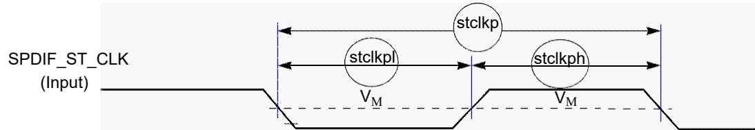
Figure 16. SPDIF_ST_CLK timing diagram
