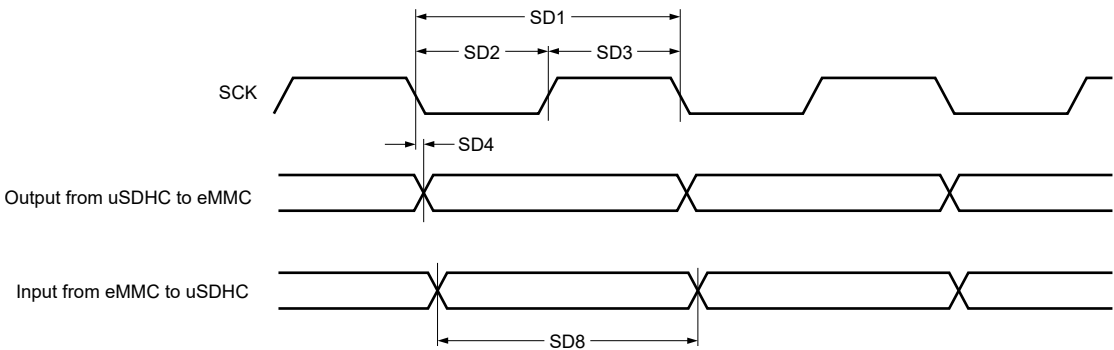
Figure 21. HS200 Mode Interface Timing
