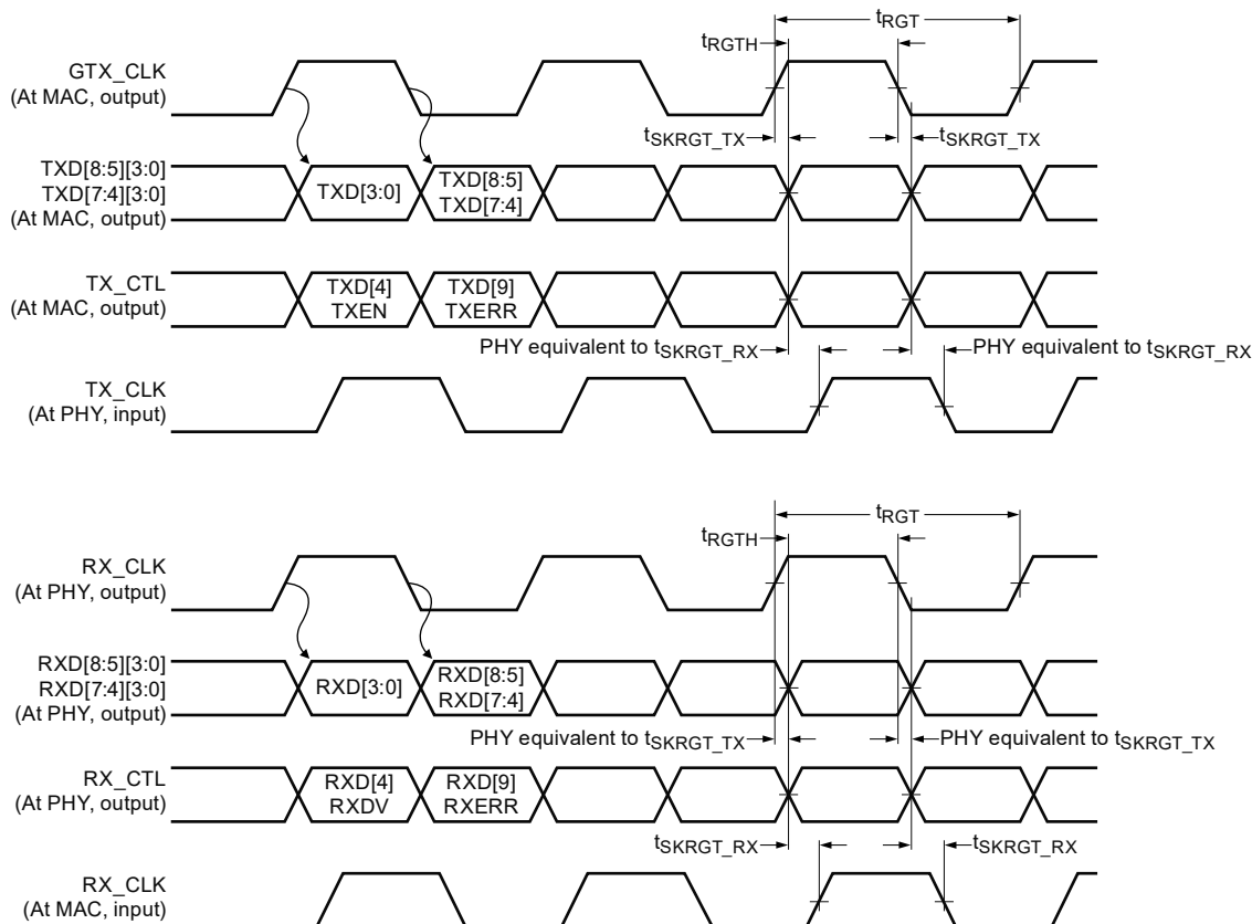
Figure 24. RGMII AC timing and Multiplexing diagram
