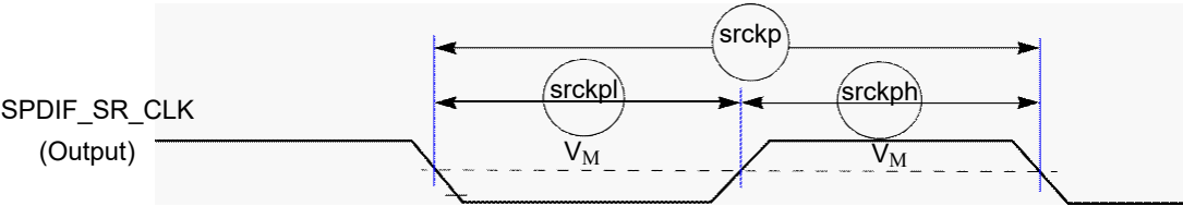
Figure 15. SPDIF_SR_CLK timing diagram
