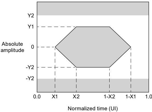
Figure 32. XFI SerDes Transmitter differential output
