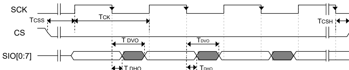
Figure 47. FlexSPI output timing in SDR mode
