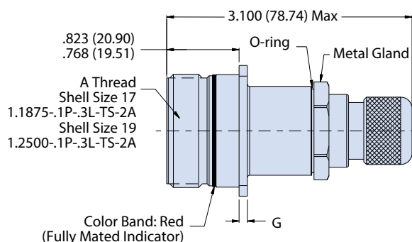
Wall Mount Receptacle Dimensions
