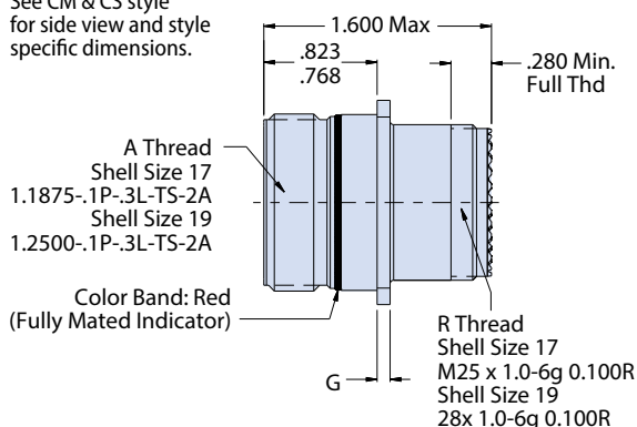
Jam Nut and Inline Receptacle Dimensions
