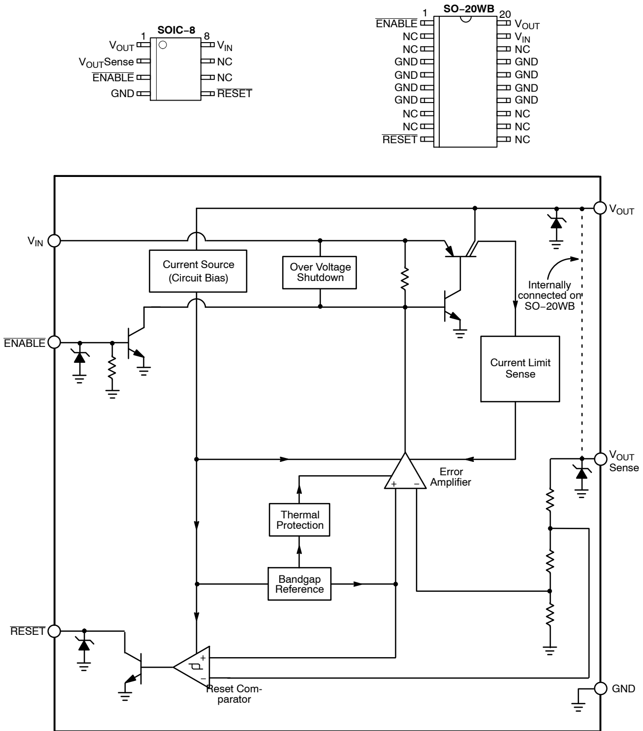
Figure 1. Block Diagram
