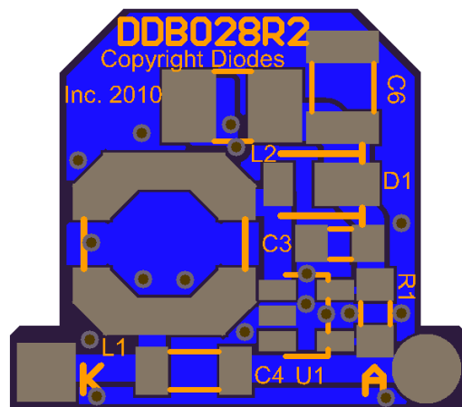
Figure 38 Bottom Layer
