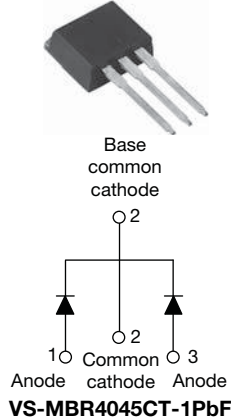
TO-262AA
