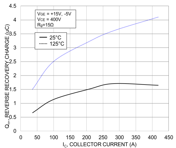
Figure 51. Typical Reverse Recovery Charge vs. I_c
