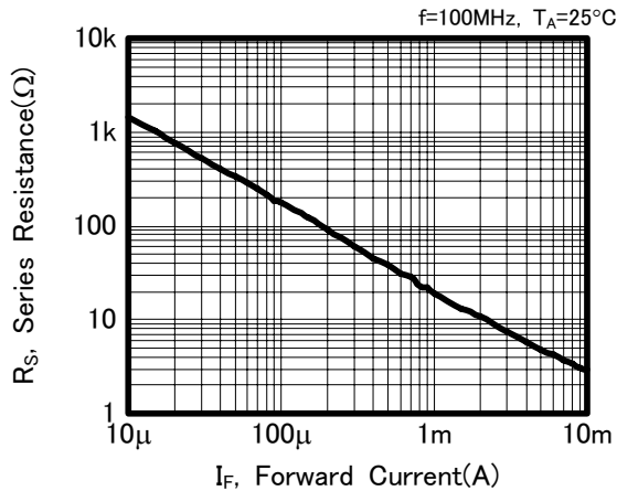
Series Resistance vs. Forward Current 順方向電流対直列抵抗
