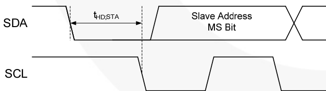
Figure 23. START Bit
