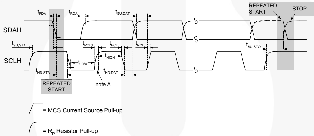
Figure 4. I²C Interface Timing for High-Speed Mode
