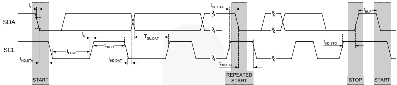
Figure 3. I²C Interface Timing for Fast and Slow Modes
