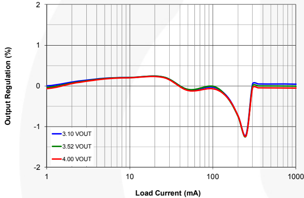
Figure 7. Output Regulation vs. Load Current and Output Voltage
