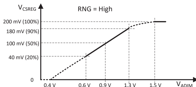
Figure 5: ADIM Pin Voltage controls the LED Current Reference Voltage with RNG = High
