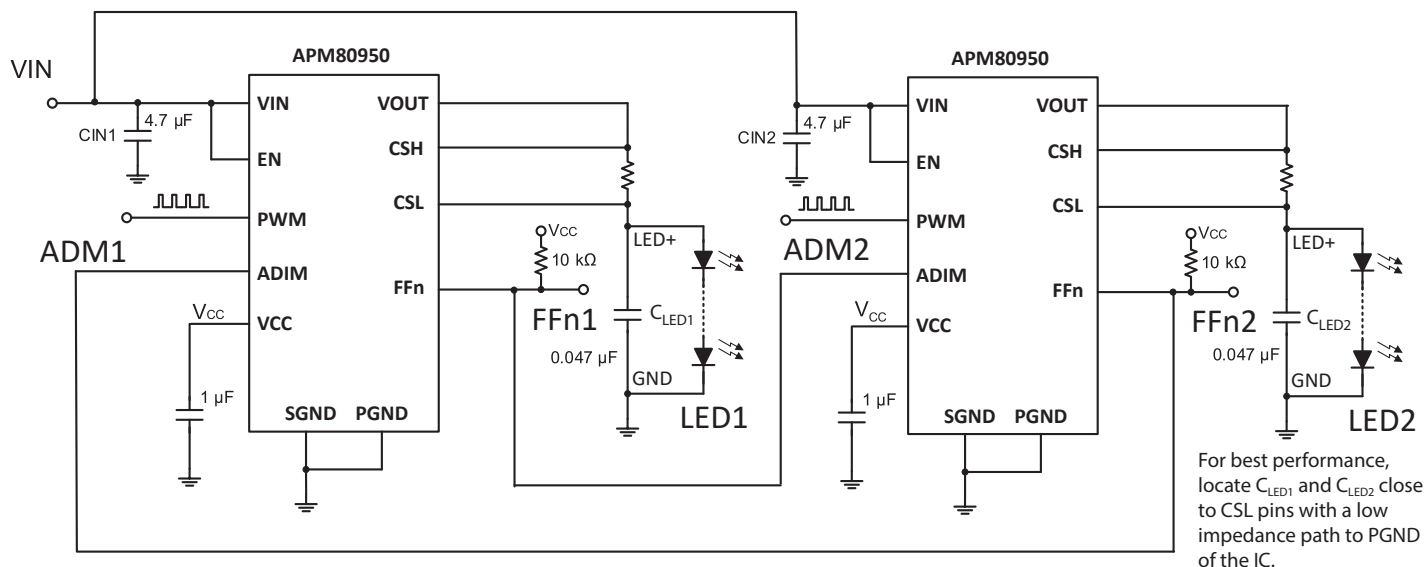
Figure 17: “One Out All Out” functionality can be implemented with 2 APM80950s driving different LED strings: When one module fails (e.g. due to LED short or open), its FFn drives other module’s ADIM Low and forces to turn OFF LED current.
