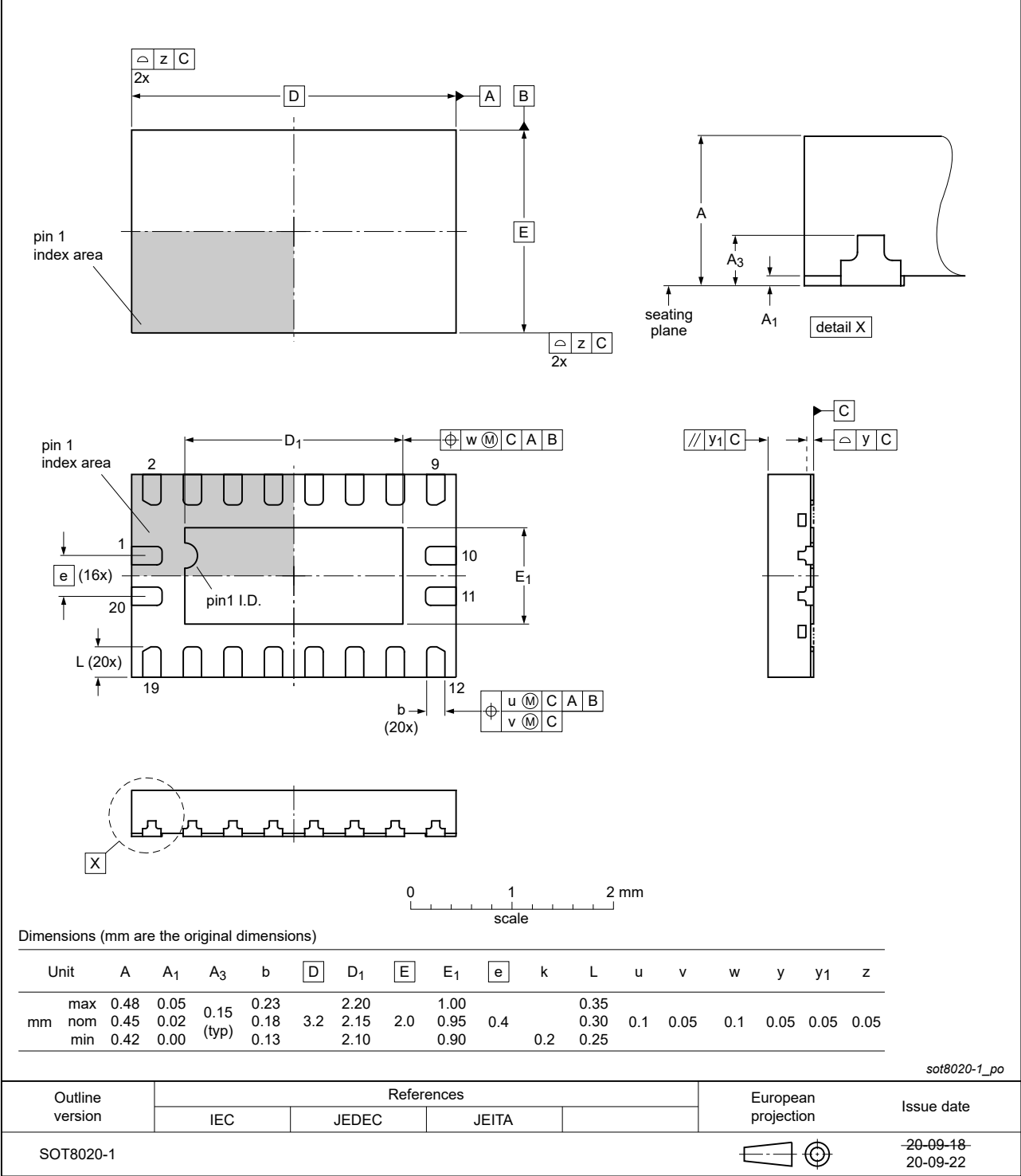
Fig. 13. Package outline SOT8020-1 (DHXQFN20)
