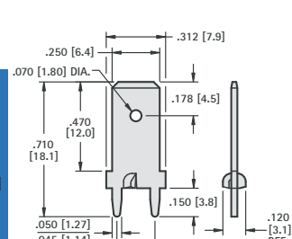
STURDI-MOUNT
