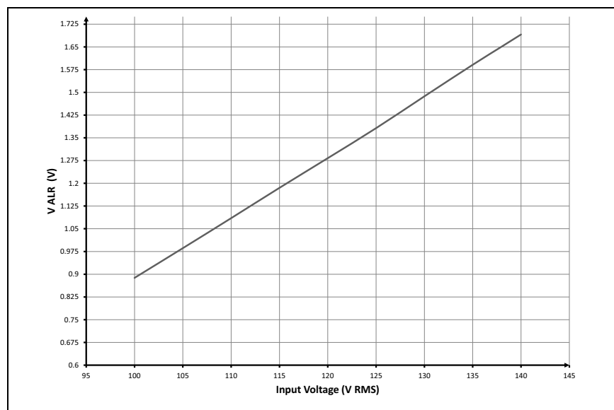
FIGURE C-21: V ALR PIN vs. Input Line Voltage.
