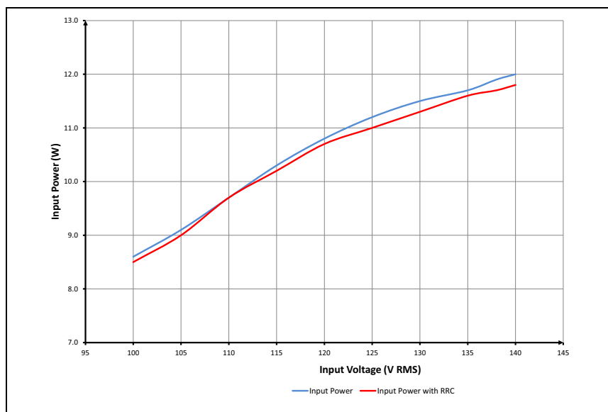
FIGURE C-17: Input Power vs. Input Line Voltage.
