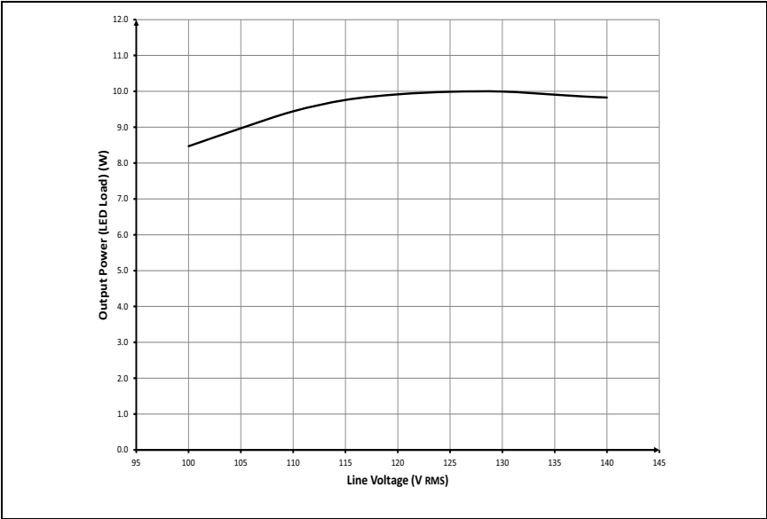
FIGURE C-22: Output Power vs. Input Line Voltage.
