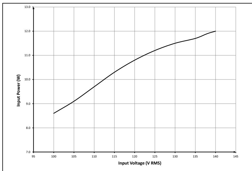
FIGURE C-16: Input Power vs. Input Line Voltage.
