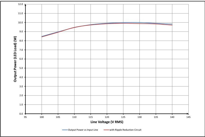
FIGURE C-23: Output Power vs. Input Line Voltage.
