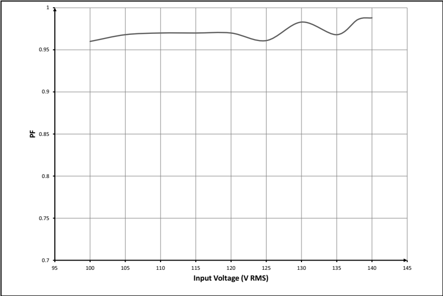
FIGURE C-18: Power Factor.
