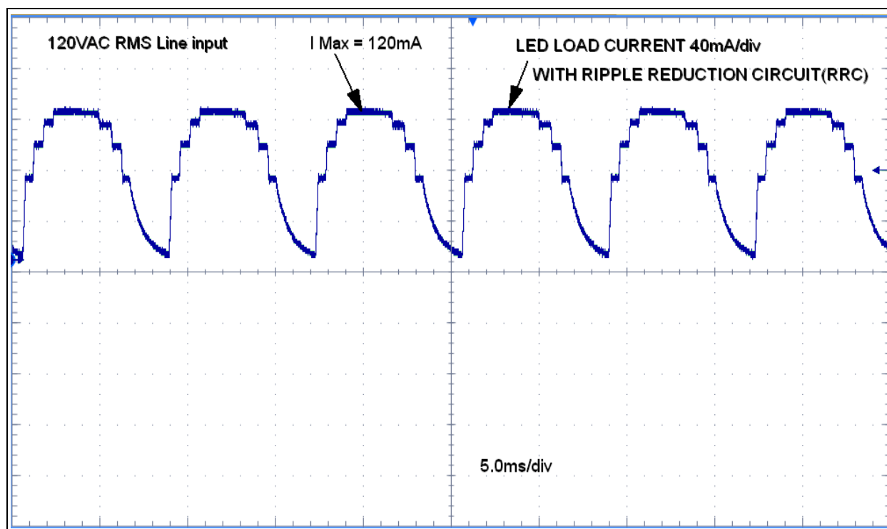
FIGURE C-14: Output Current with Ripple Reduction Circuit on 120 V AC RMS Input.
