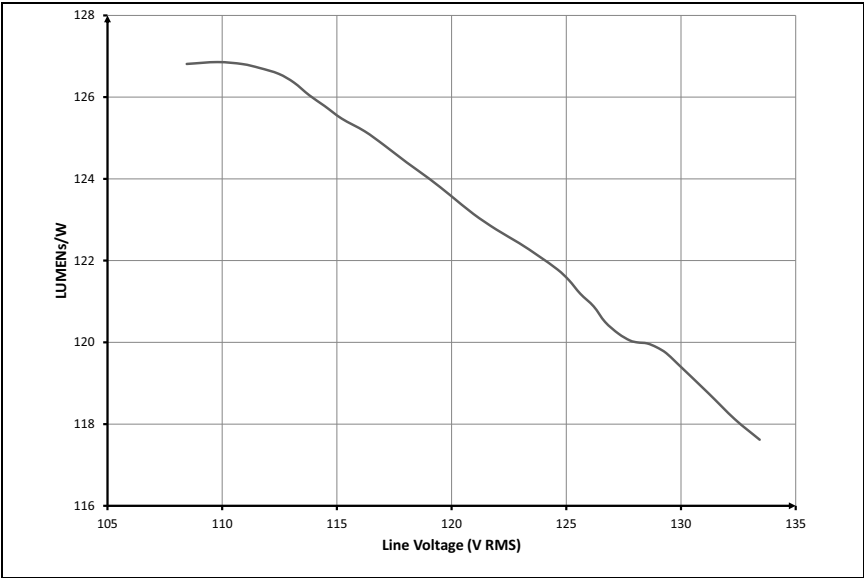
FIGURE C-27: Efficacy.
