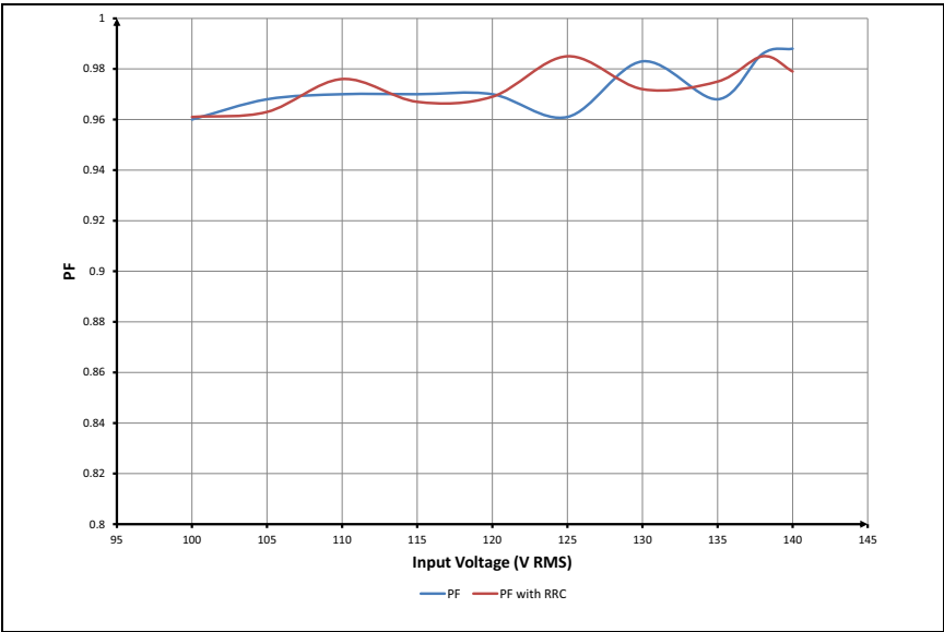
FIGURE C-19: Power Factor.
