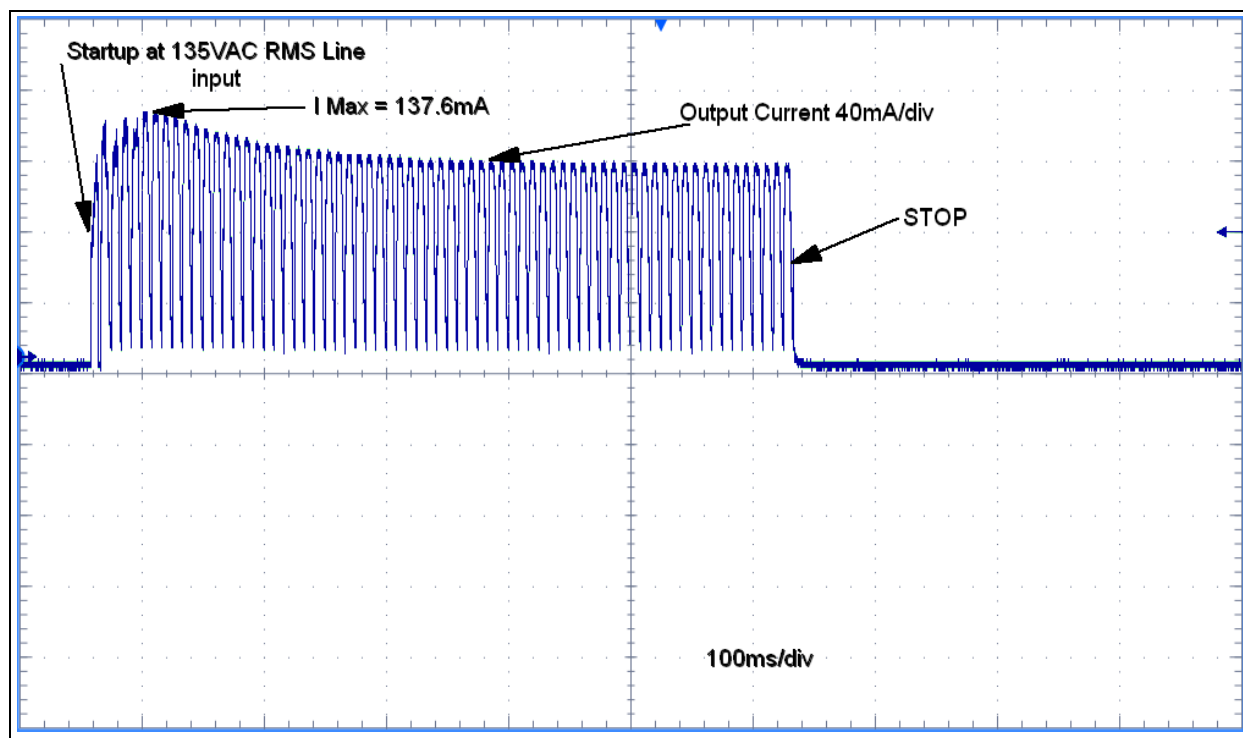
FIGURE C-10: Output Current on Startup at 135 V AC RMS Line Input.
