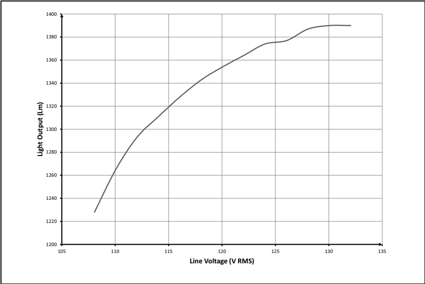
FIGURE C-26: Light Output vs. Input Line Voltage.
