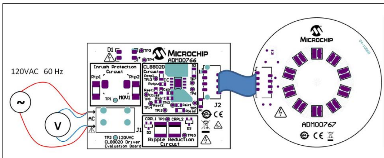
FIGURE 2-1: Connection Diagram.
