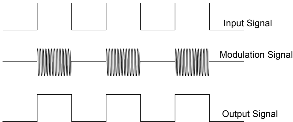
Figure 7. Modulation Scheme
