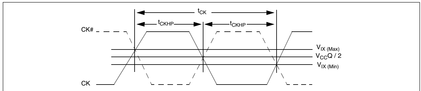
Figure 32 Clock characteristics
