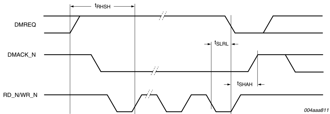
Fig 20. Burst DMA timing
