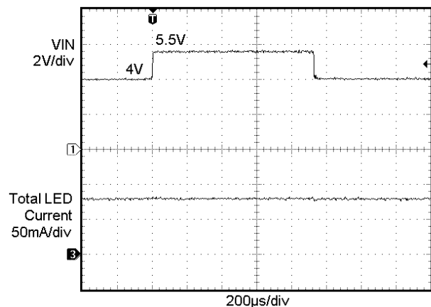
Figure 15. Line Transient Waveform 4 V to 5.5 V
