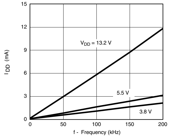
Supply Current vs. Frequency
