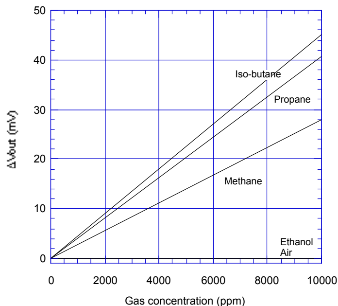
Sensitivity Characteristics:
