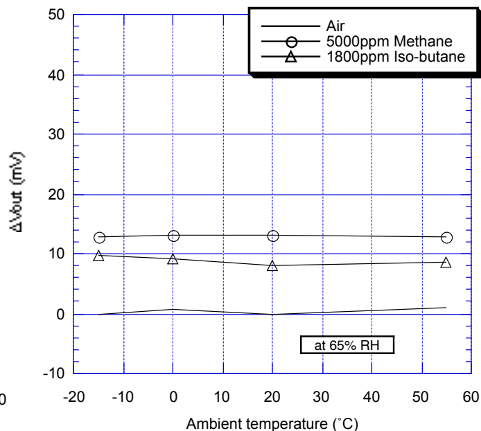
Temperature Dependency:
