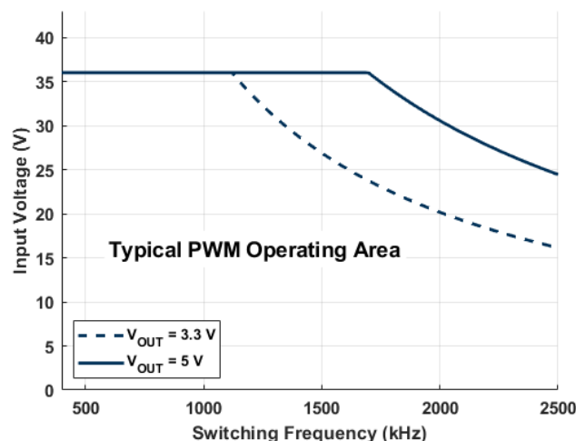
Figure 8: Input Voltage Limit To Prevent Pulse Skipping
