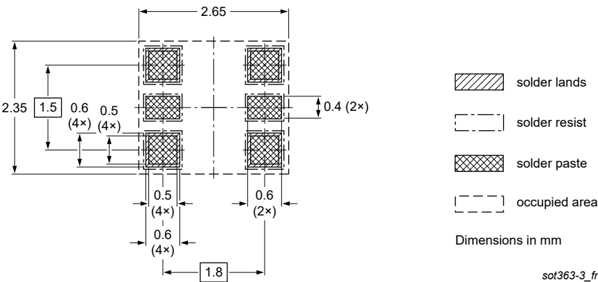
Fig. 5. Reflow soldering footprint for TSSOP6 (SOT363-3)
