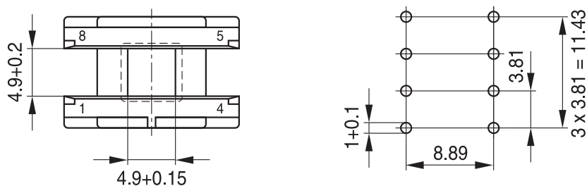
Hole arrangement View in mounting direction
