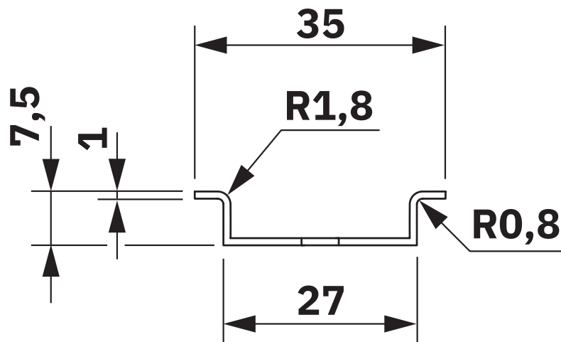
Dimensional drawing
