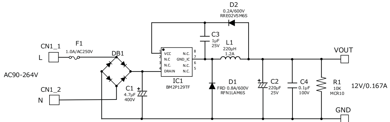
Figure 23. BM2P129TF-EVK-001 Schematics
