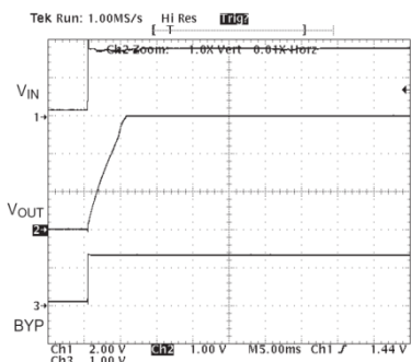
Fig. 18: Fast V_{IN} , C_{OUT} =1000µF, I_O =500mA
