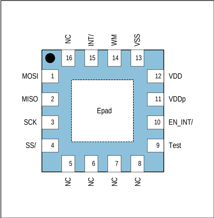
Figure 3: Pin Diagram
