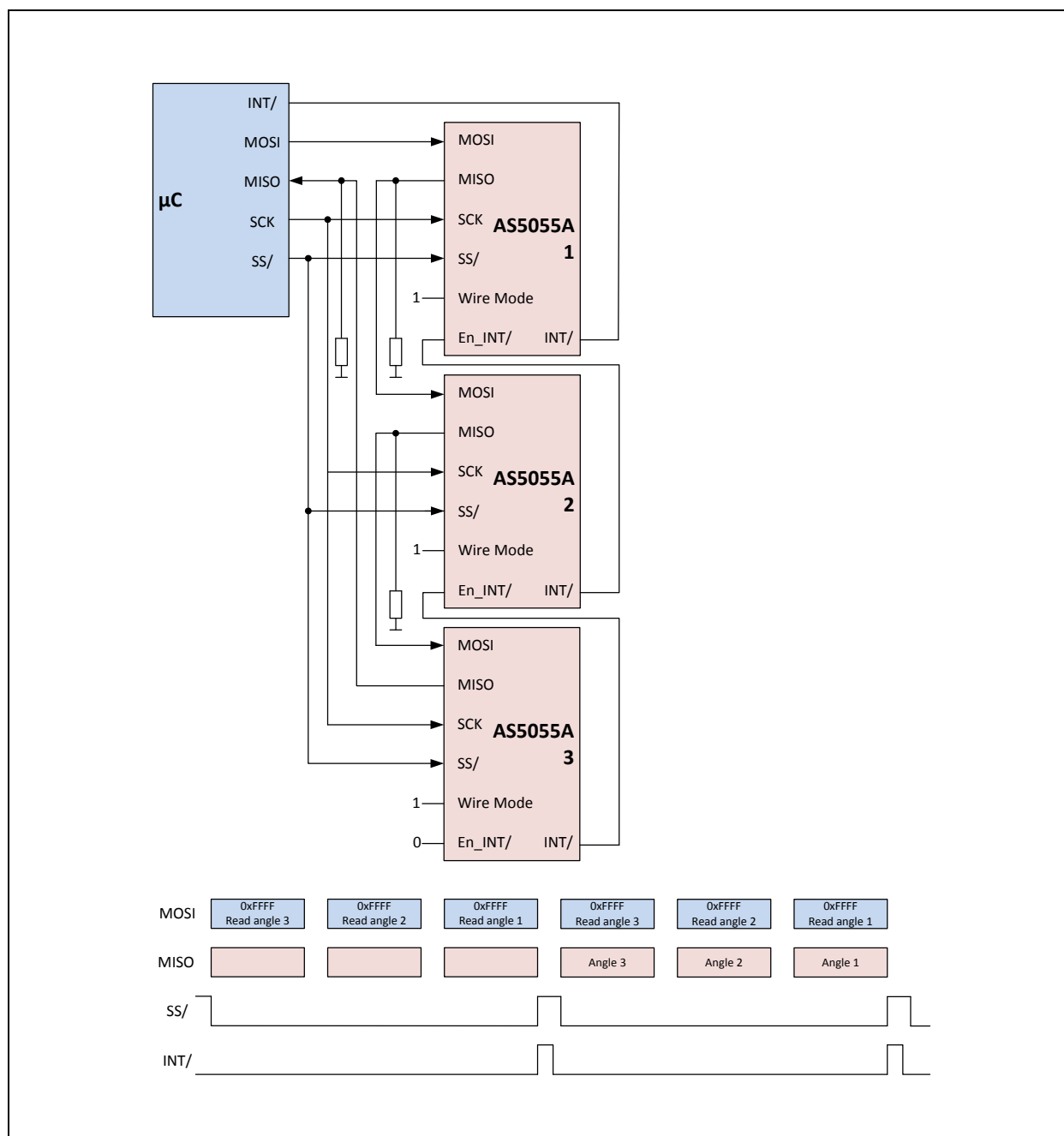
Figure 21: Daisy Chain, 4 Wire
