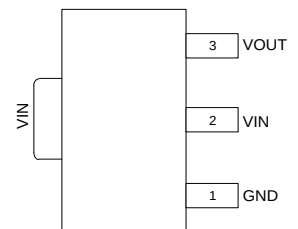
SOT89 (AP7387-XXY-13)
