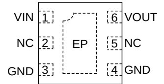
U-DFN2020-6 (Type C) (AP7387-XXFDCR-7)
