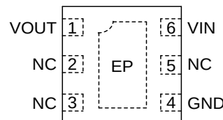
U-DFN2020-6 (Type C) (AP7387-XXFDC-7)
