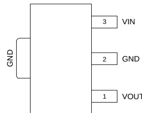
SOT89 (AP7387-XXYR-13)
