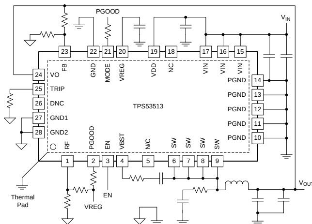
Simplified Schematic
